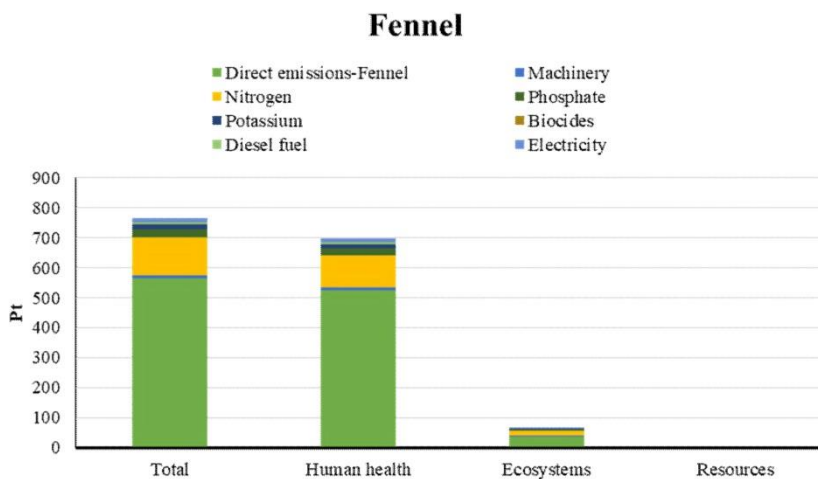
Figure 4. Weighting results of the damage categories in cumin and fennel production.
